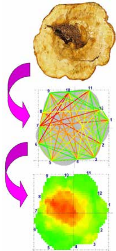
Figure 3. Commonly, the direct distance between the sonic sensors is divided by the measured time-of-flight and this virtual speed is visualized by using different colors: green for the highest, red for low speed values. The red lines, however, do not represent the travel path of the measured waves because they made a detour around a defect. In this kind of sonic tomography, invented in 1999, the arrival time of the quickest arriving signals is measured and these waves typically travel on a detour through the intact parts of the cross-section, thus around defects.
