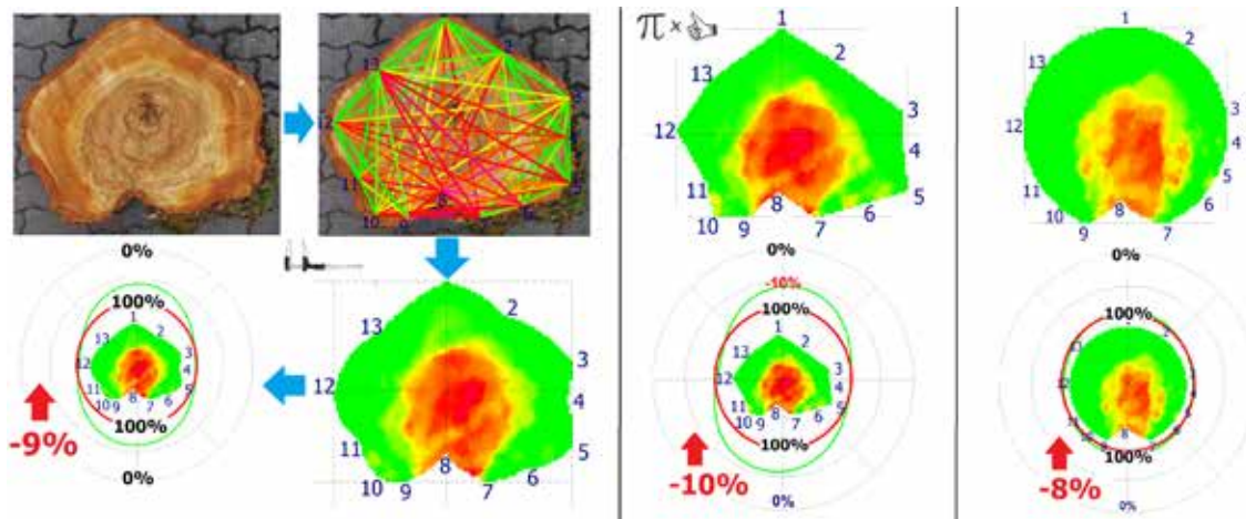
Figure 8. Precise sensor positions ( \Delta \leq 1\text{cm} ) lead to a loss in section modulus and thus load-carrying-capacity of this defective cross-section of \sim 9\% (left). Rounding sensor positions and radius differences to 5cm units ( \Delta \leq 5\text{cm} ) results in \sim 10\% (middle). Ignoring radius differences for all except one sensor, thus assuming a practically circular cross-section (right), leads to \sim 8\% estimated loss in load-carrying-capacity. In this example, maximum sensor position exactness, thus does not lead to a significantly different final result as compared to the quick and simple approaches.
