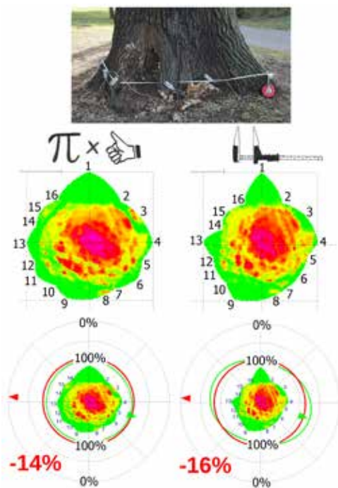
Figure 9. At this oak ( Quercus petraea ), a tree-risk expert, who was not yet experienced in sonic tomography, first recorded the positions of the sensors using a measuring tape (left) and guessing radius differences. Then, the sensor positions were determined precisely by using a caliper (right). Although the two cross-sections look different, the final and most important result of the assessment (=relative loss in load carrying capacity) did not vary significantly by increasing the accuracy of the sensor positions. In terms of a risk evaluation, there is not much of a difference between 14 and 16% loss in cross-sectional load-carrying-capacity.
